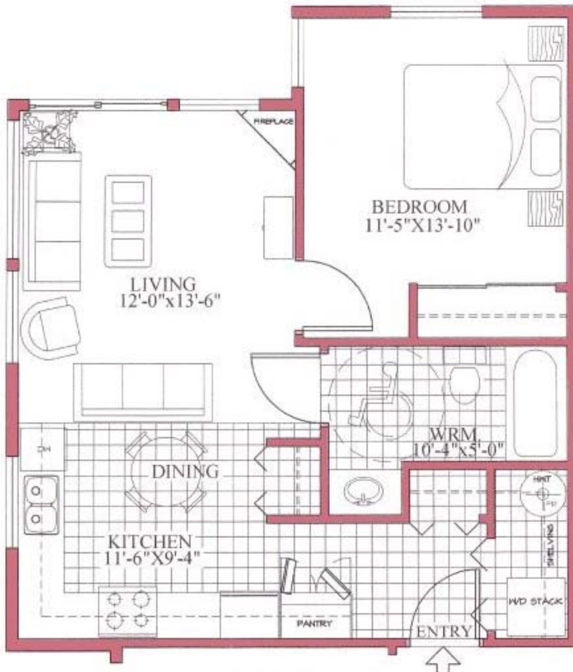
UNIT "A" FLOOR PLAN (1 TOTAL) SCALE 1/4" = 1'-0" 588 SQ. FT. 54.6 m2 1 BEDROOM SUITE 106
